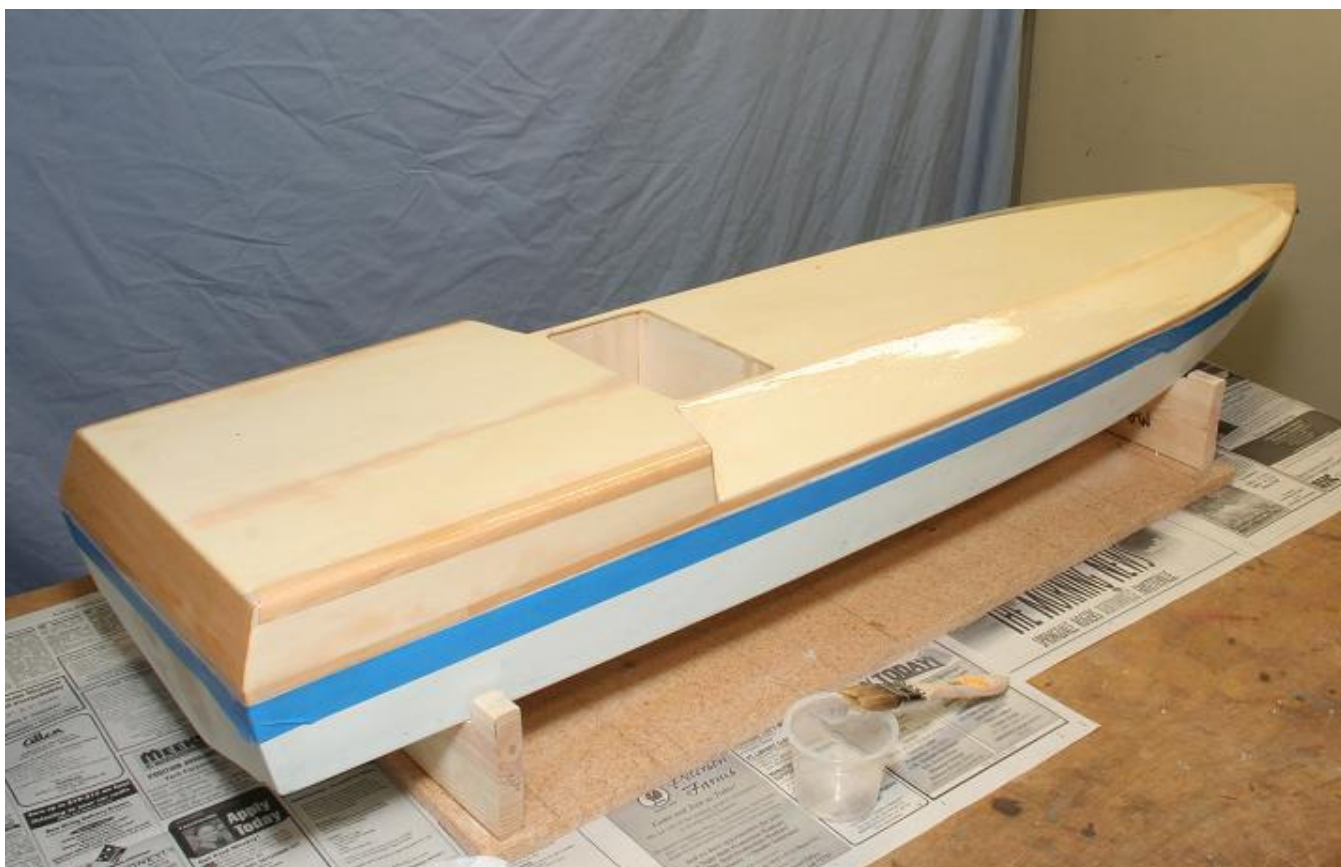
Patched the transom, sheathed in plywood, & two coats of epoxy
