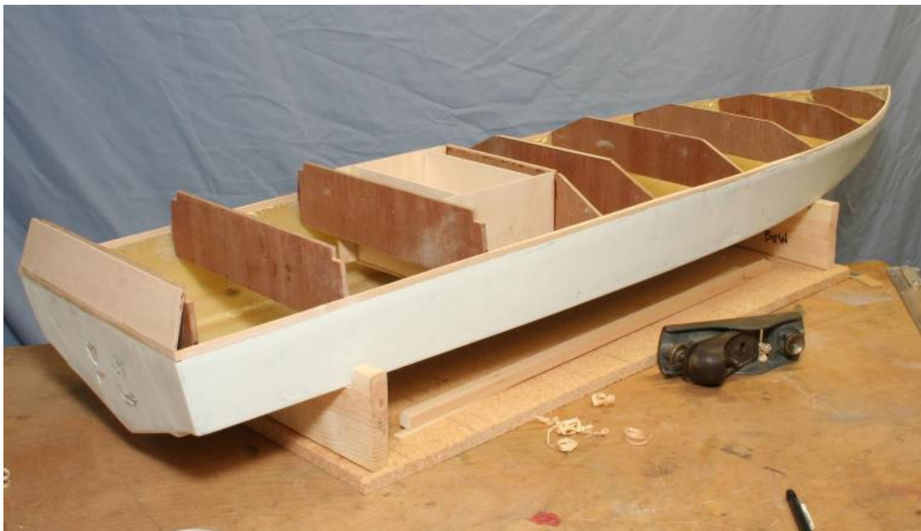
New frames and gunwale strip
