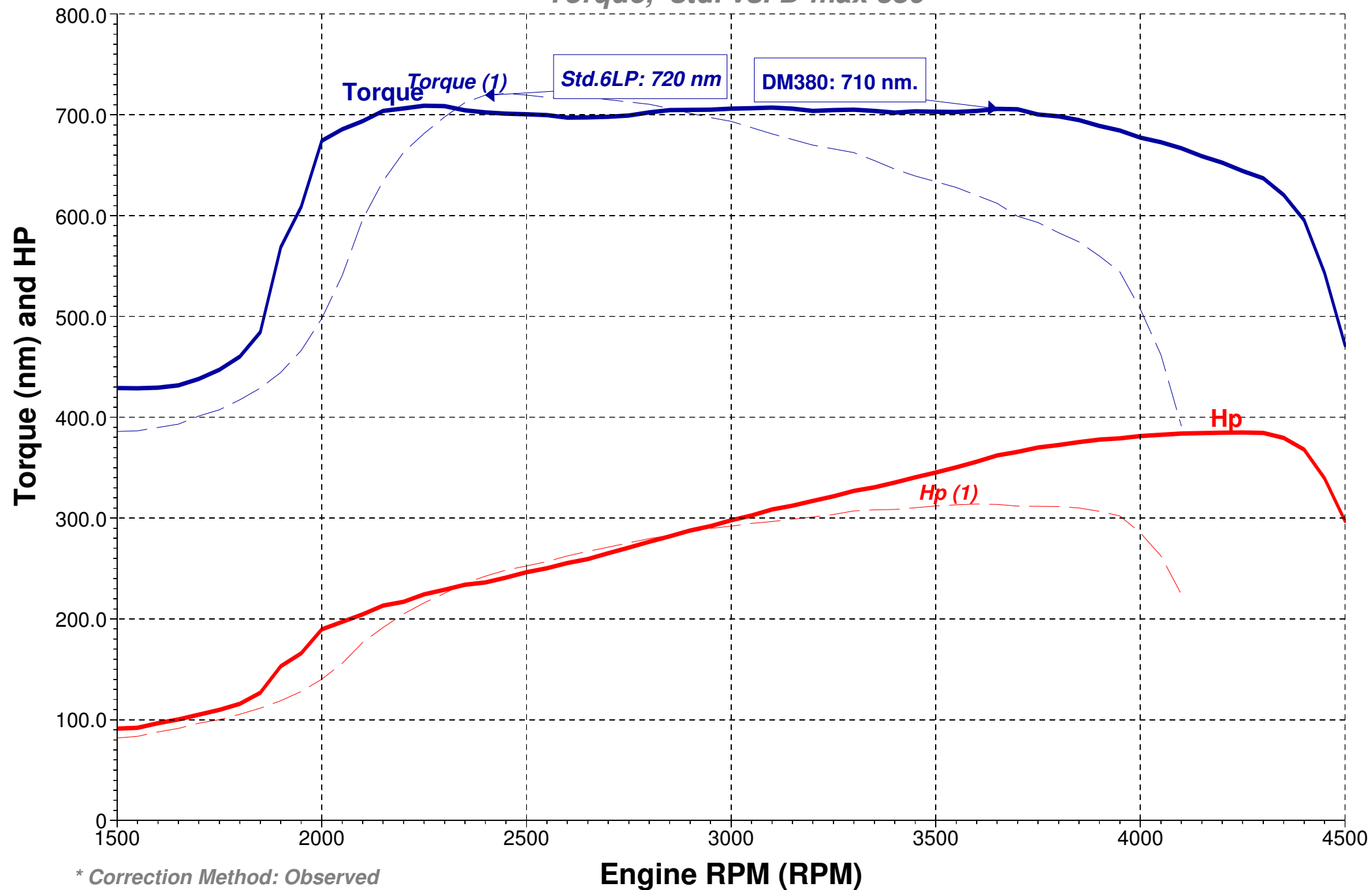
Torque, std. vs. D-max 380
