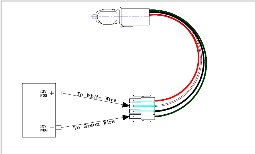
Diagram "A" Four-Wire Solenoid Pull Coil Test
