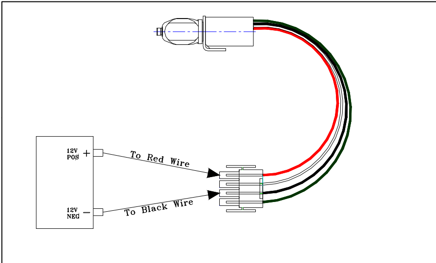
Diagram "B" Four-Wire Solenoid Hold Coil Test
