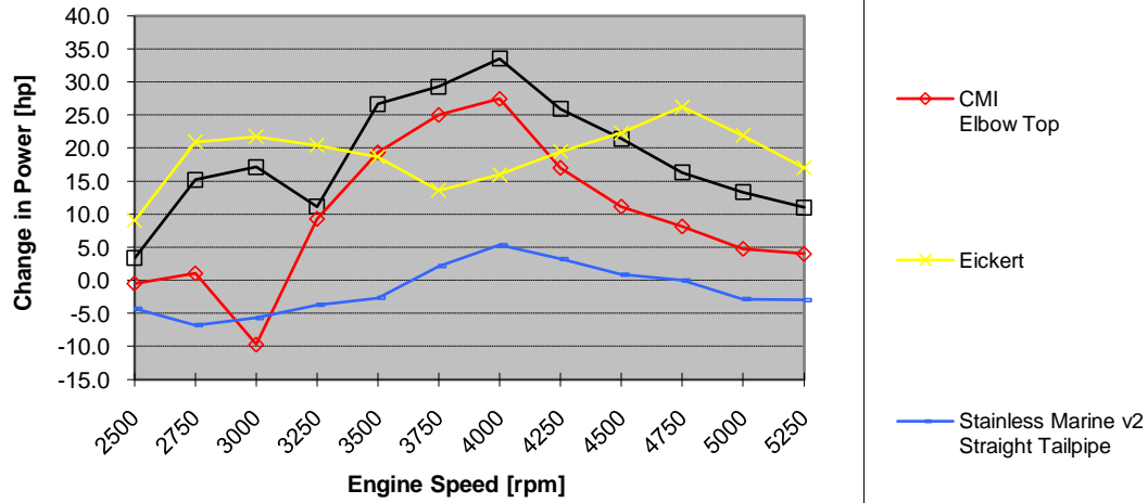
Fountain 500 Exhaust Comparison Change in Power Using Stainless Marine v1 as Baseline
