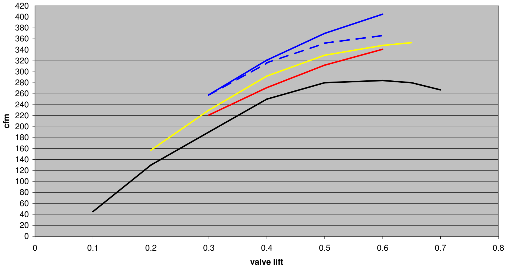
Intake CFM - Various GM Gen 7 heads
