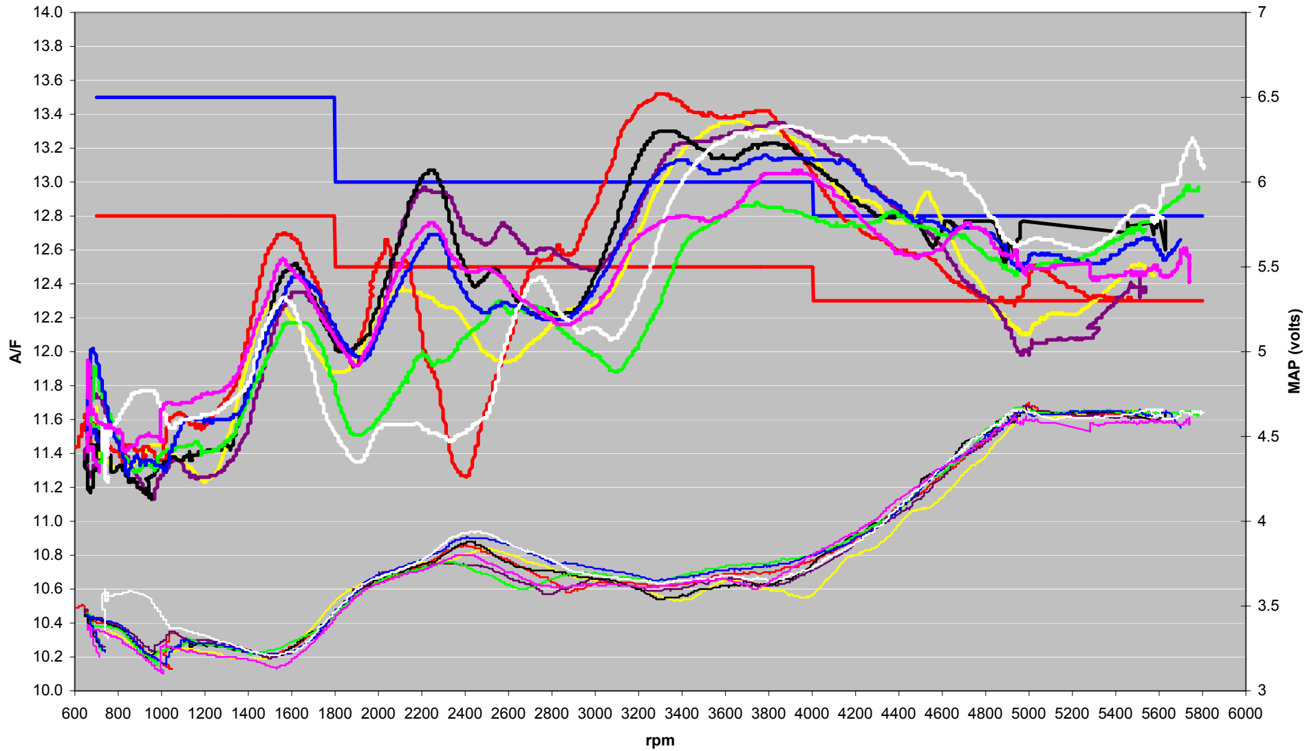
A/F vs MAP vs RPM @50psi fuel , Cal #A8 7-16-2008 [4.18 sec (max) Smoothing]
