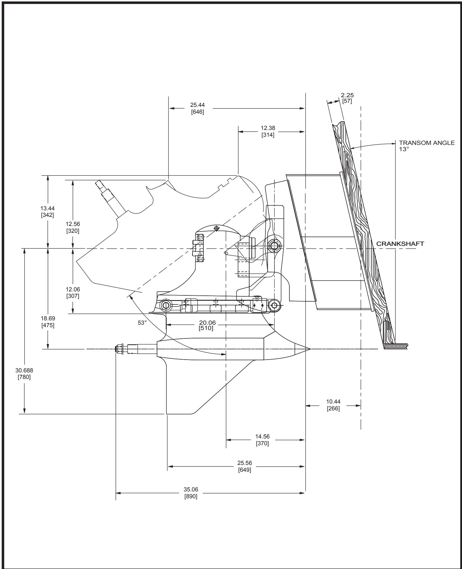
V SSM Drive with Stand-Off Box
